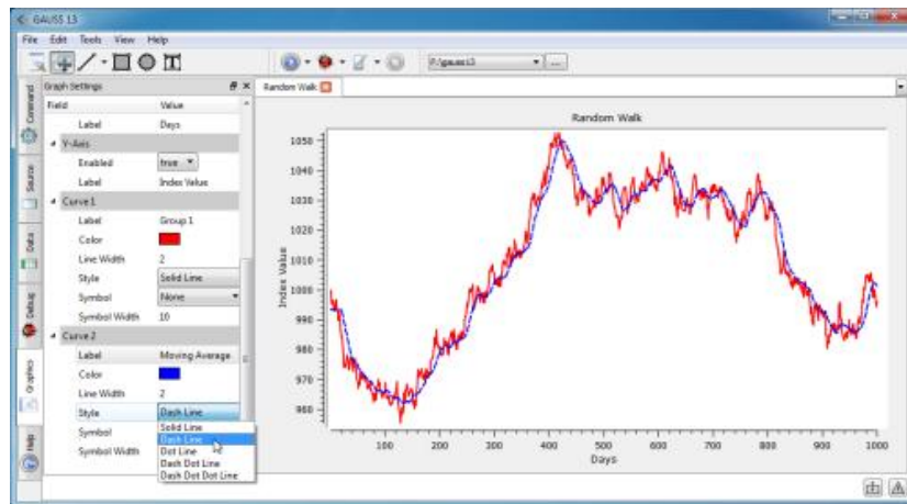
Figure 7.1: Changing Appearance
