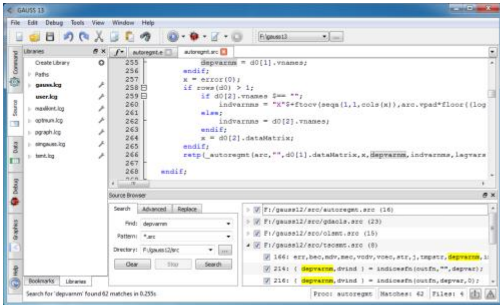
Figure 3.23: Source Browser
