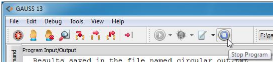
Figure 3.39: Stop
