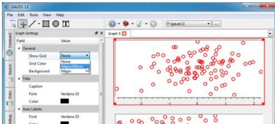
Figure 7.7: Highlighted Object
