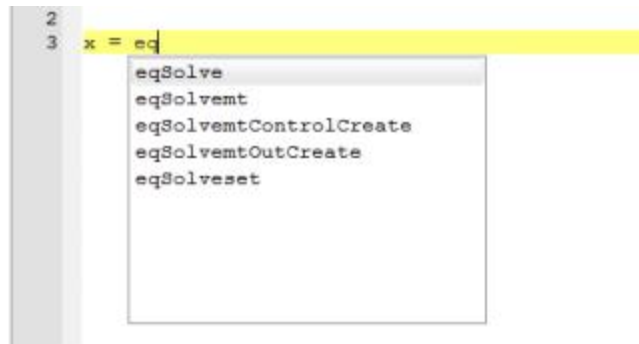
Figure 3.13: Autocomplete
