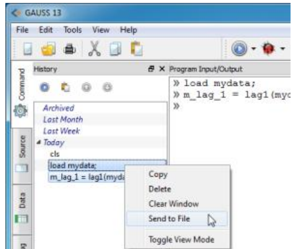
Figure 3.9: Command History
