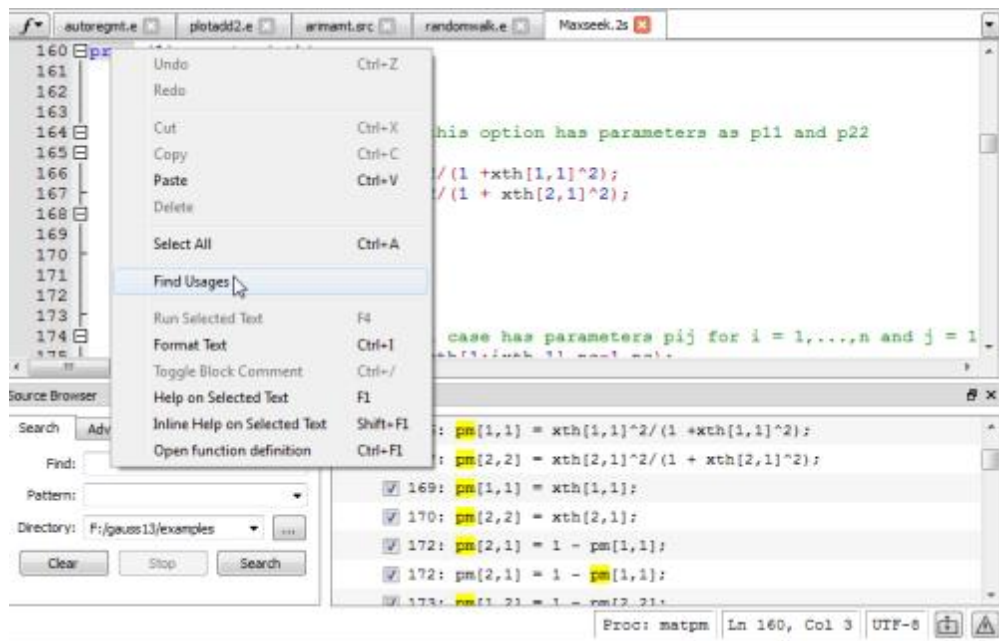
Figure 3.18: Find usages
