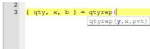
Figure 3.14: Tooltips
