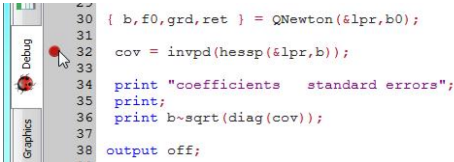
Figure 3.35: Setting Breakpoints
