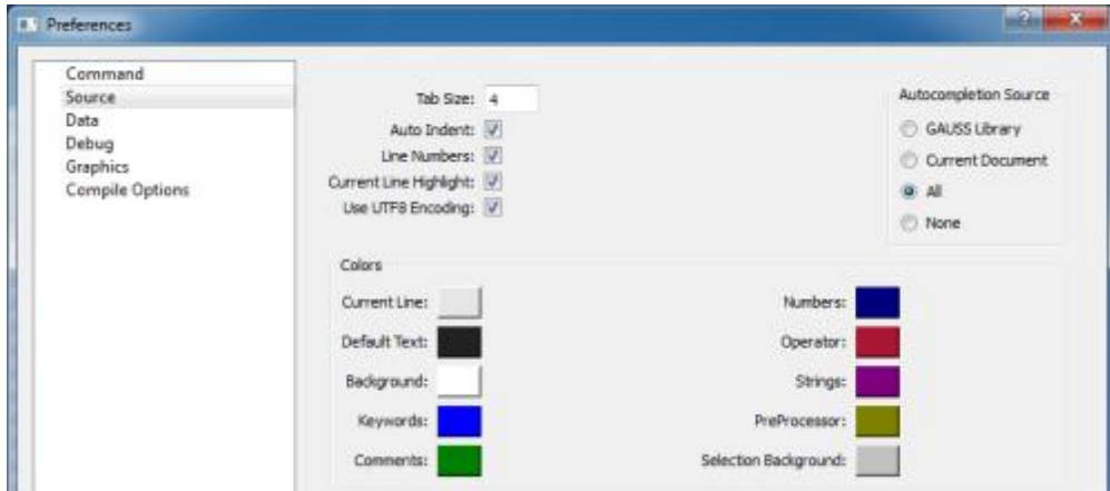
Figure 3.21: Editor Preferences
