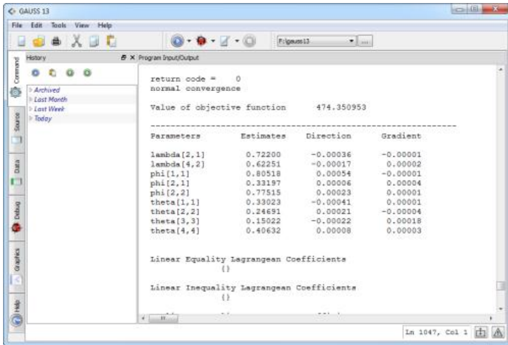
Figure 3.1: GAUSS page organization
