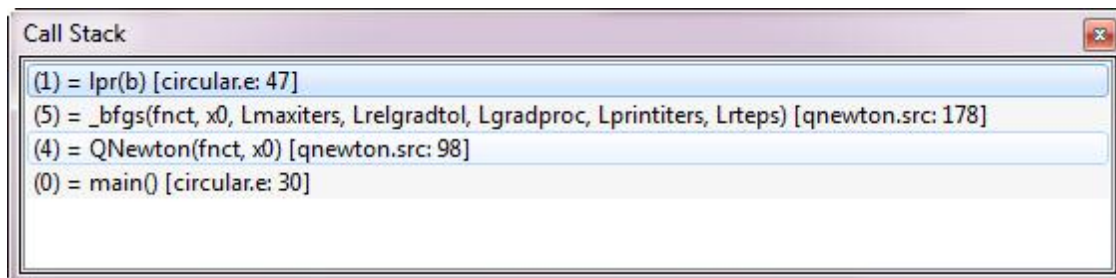
Figure 5.6: Call Stack Window
