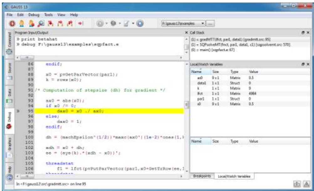
Figure 5.2: Debug Window
