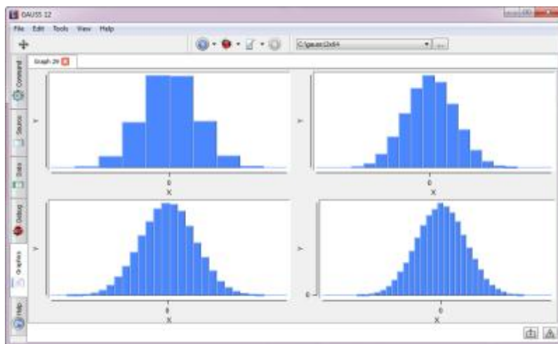
Figure 6.9: Example Subplot
