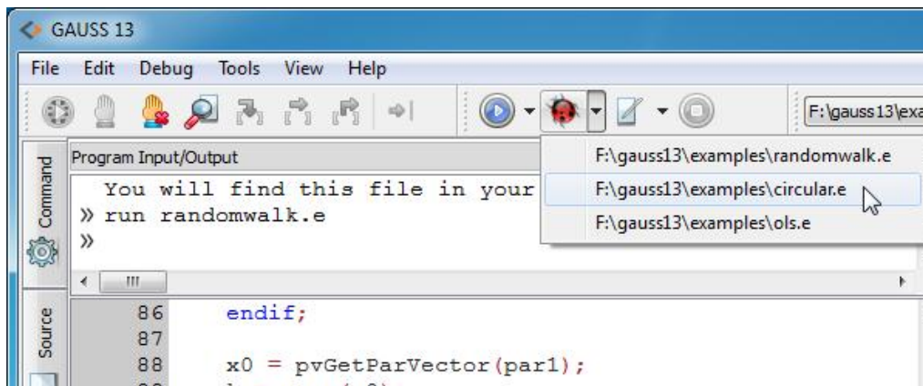
Figure 3.34: Debug Button
