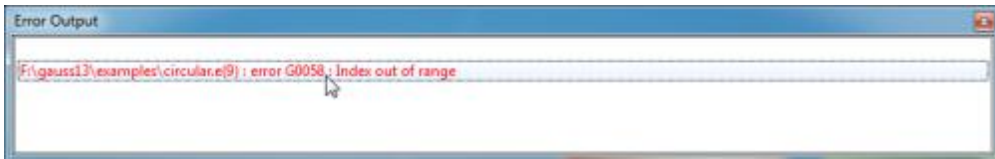
Figure 3.10: Error Window
