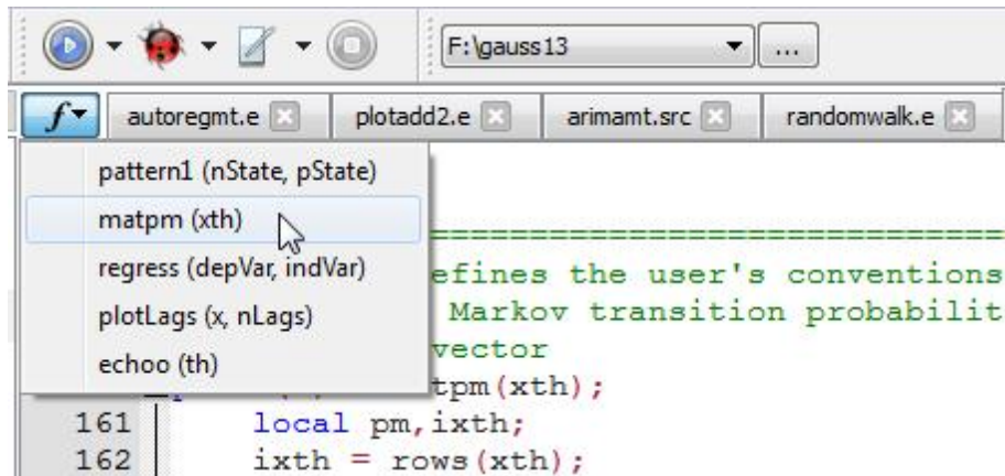
Figure 3.15: Function Browser
