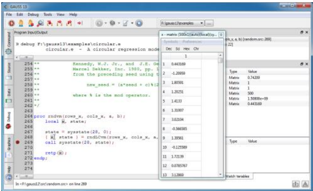
Figure 3.40: Watch Window
