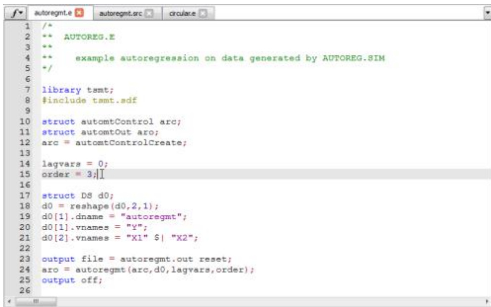
Figure 3.12: Programming Editor
