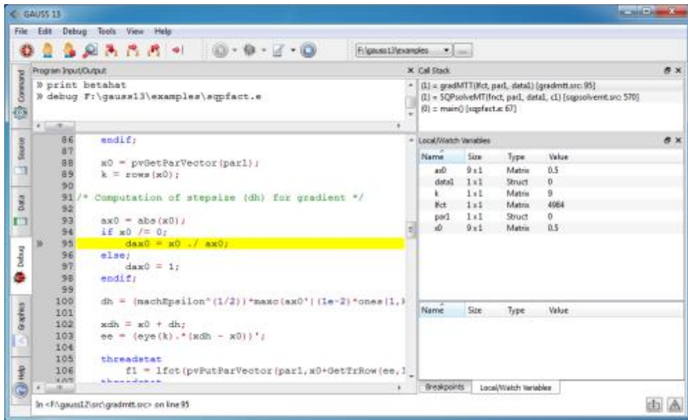
Figure 3.33: Debug Window
