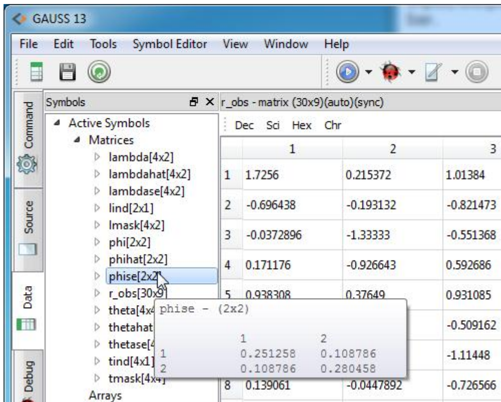
Figure 3.29: Symbol View
