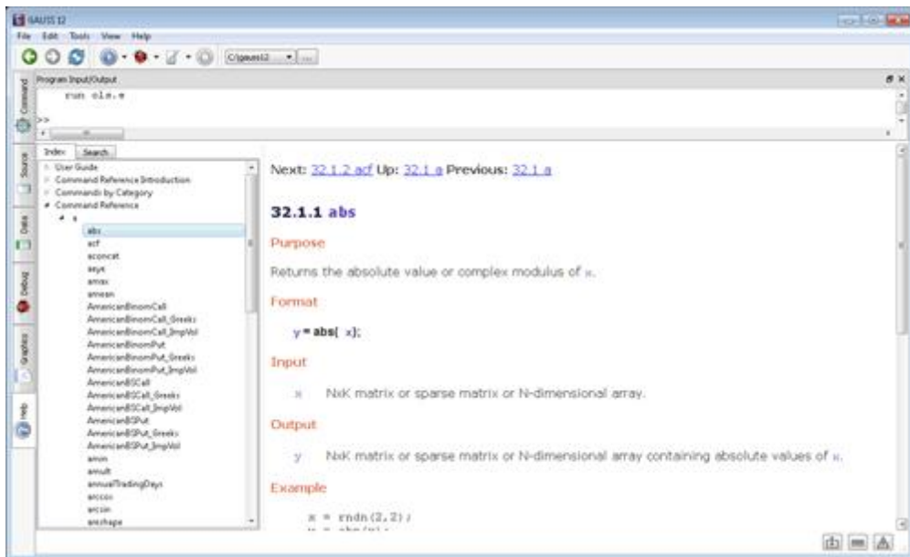
Figure 3.41: Help Page
