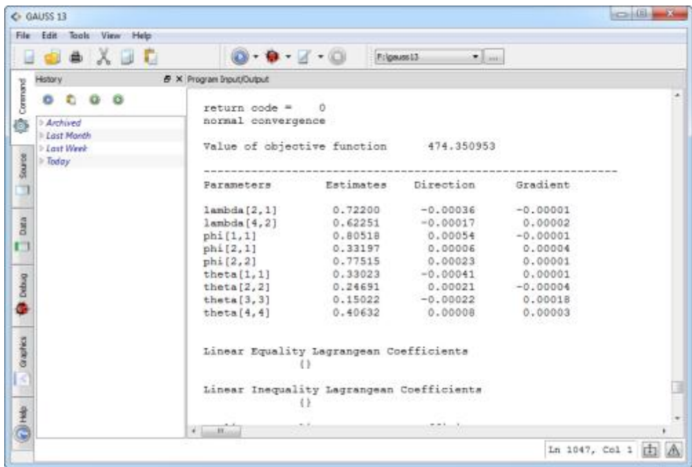
Figure 3.2: Command Page
