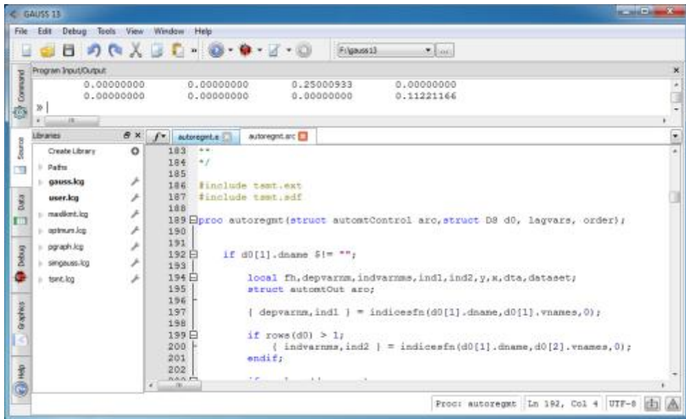
Figure 3.11: Source Page
